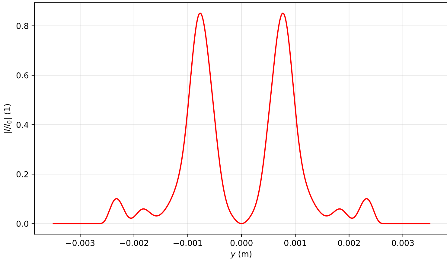
Intensity profile I(x = 0, y, z = 3.662)/I_0 , P_{in}=5.0P_{cr} , artificial time
